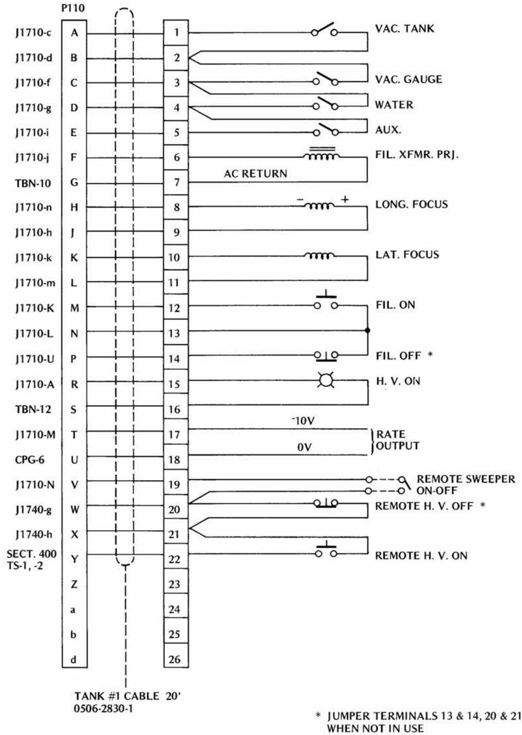
Figure 2-4. CV-14 A and B interlock terminal strip connection diagram
